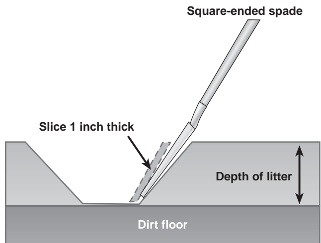
Figure 2. Using the point method with a square-ended spade, first dig a small trench before removing the sample. This ensures that equal amounts of litter are removed from all depths.
